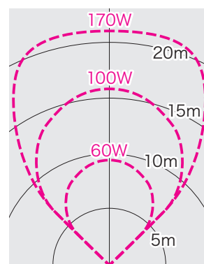
PDS-C04-60FL(60W型) PDS-C04-100FL(100W型)
